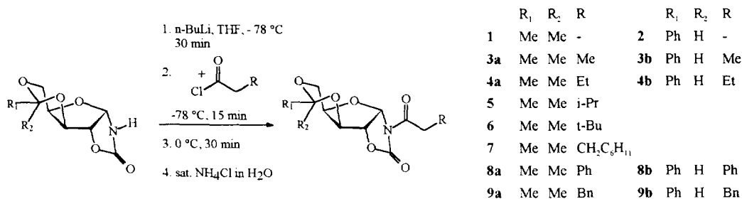
Figure 1 : standard N-acylation sequence 2
