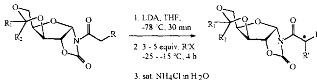
Figure 3 : \alpha -alkylation reaction
