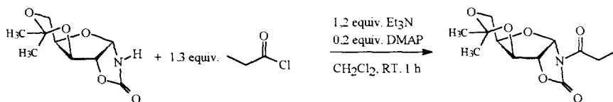
Figure 2 : exemplary N-acylation procedure converting 1 to 3a (92 %) using catalytic amounts of DMAP
